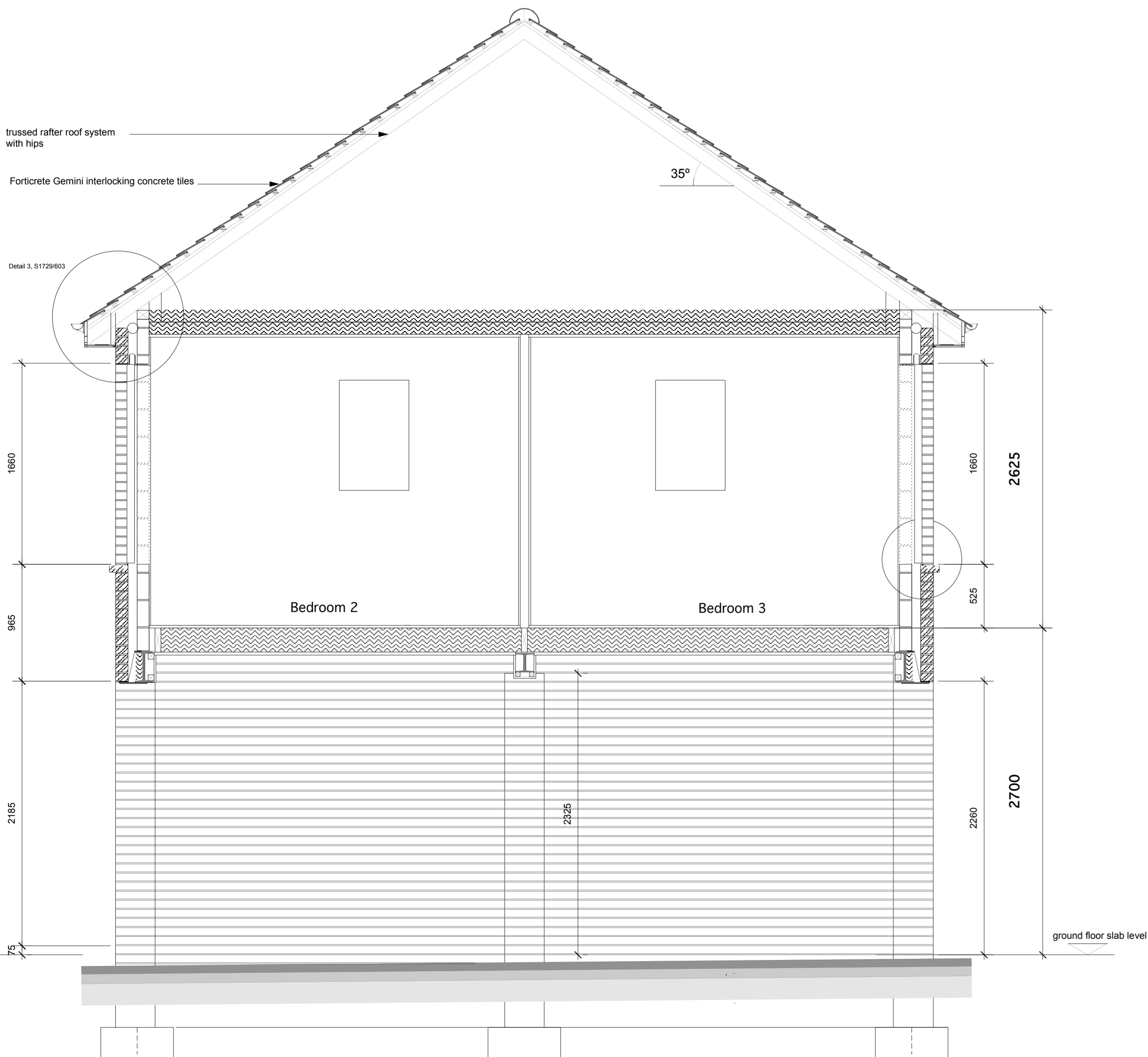
SECTION BB
