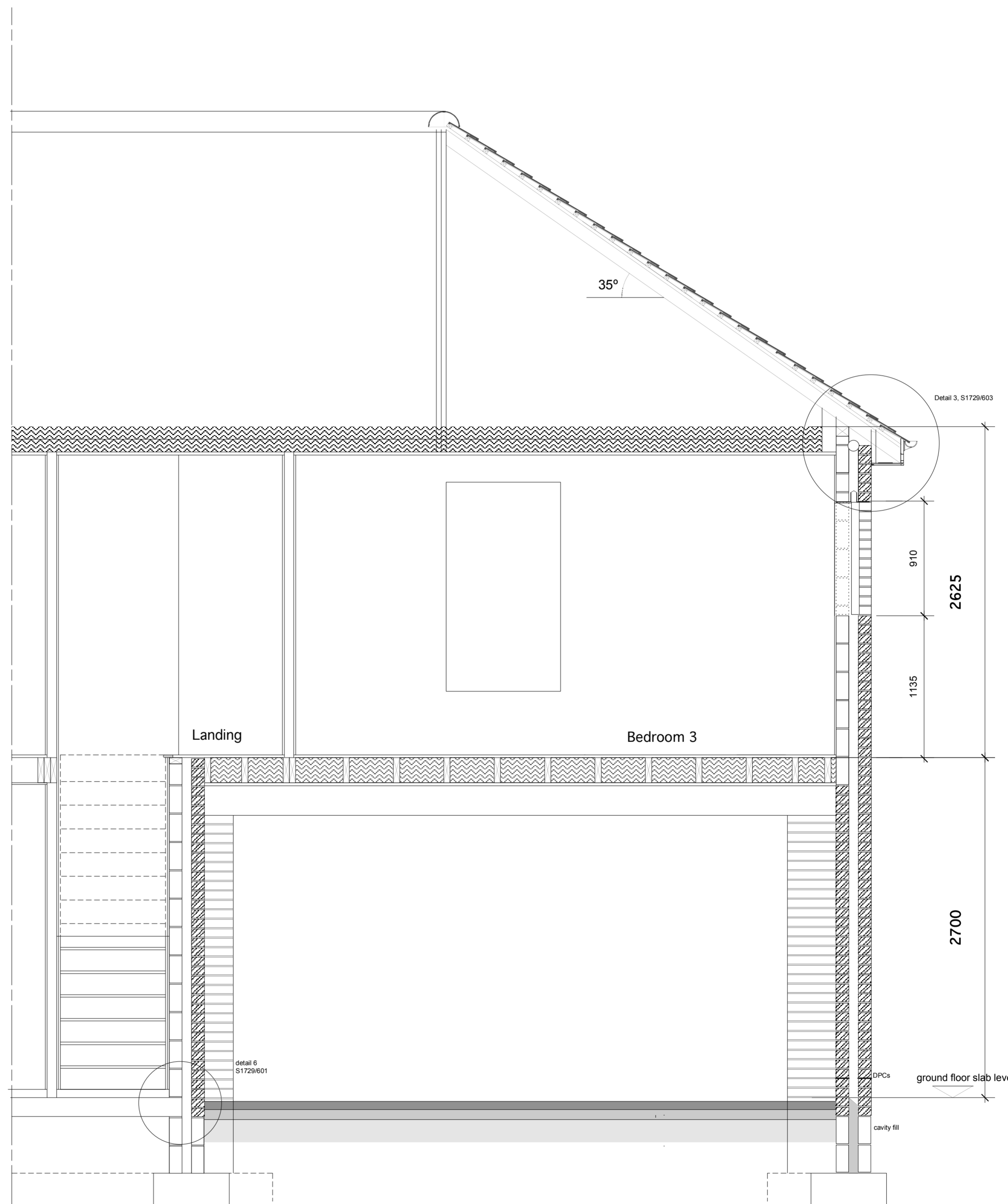
SECTION CC
